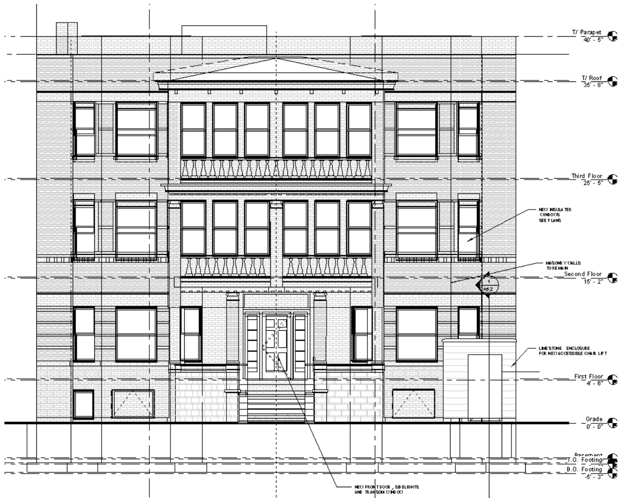
West Elevation
